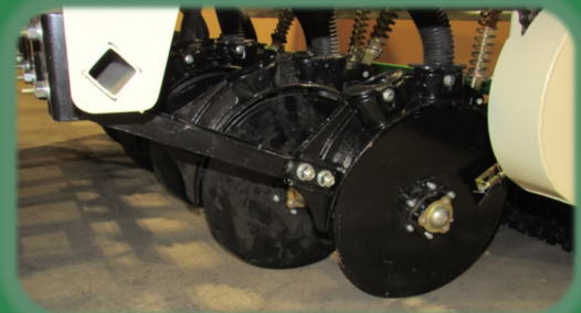
Double Disc Openers, Allowing Front Hopper To Plant In Rows
