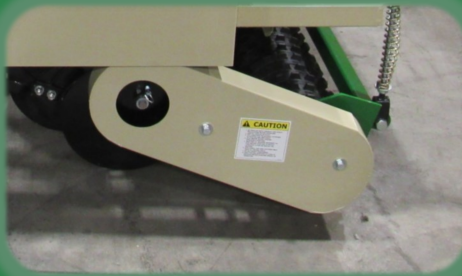
Shearpin for Seedcup Safety Can Also Be Pulled Out To Disengage Seeding System For Use As An Aerator
